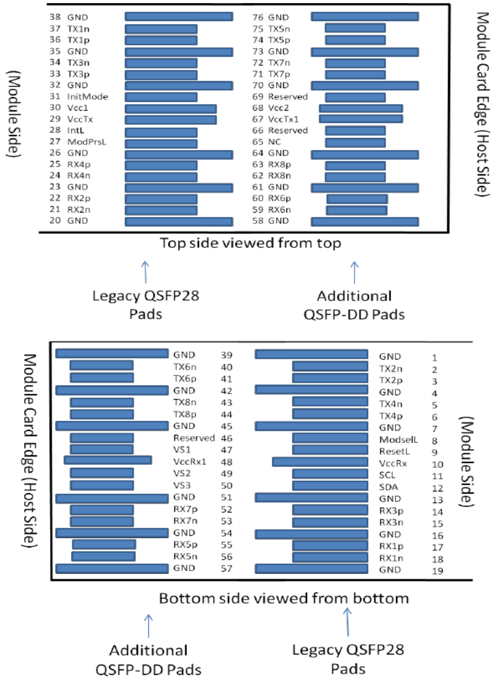
Figure 3 MSA Compliant Connector
